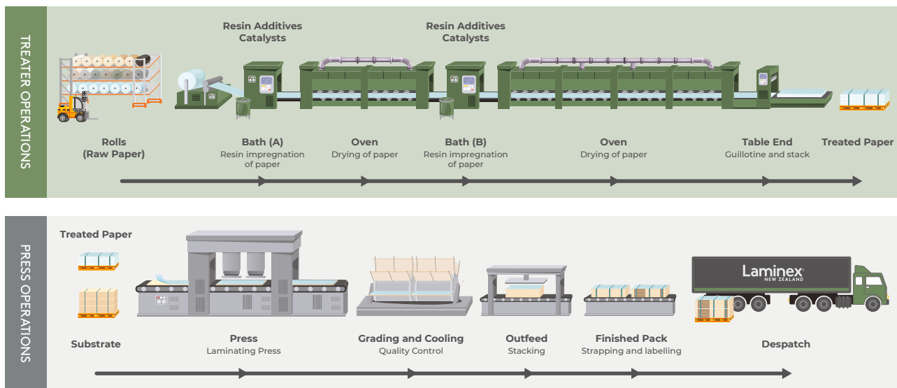
Figure 1: Melteca® and Whiteboard Manufacturing Process
